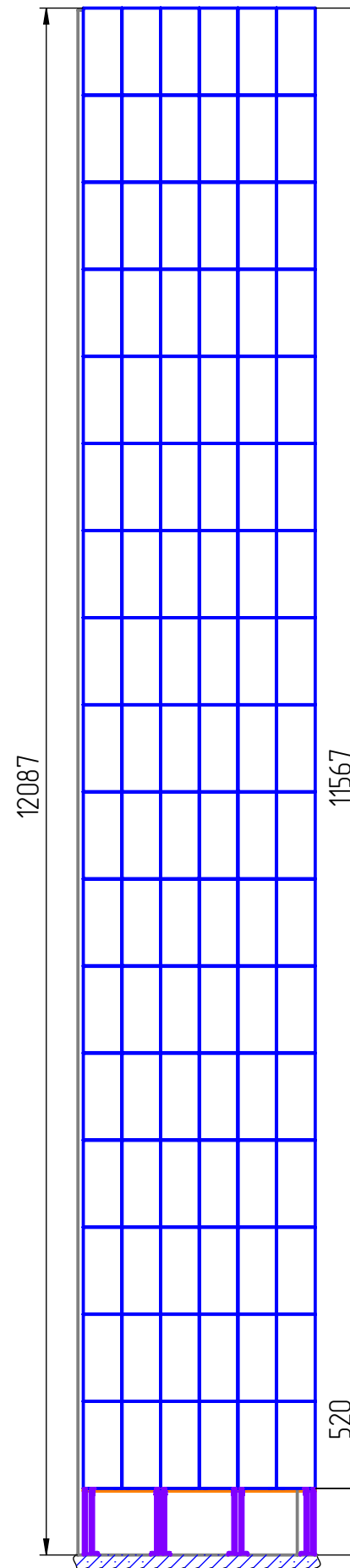
1-1 (1:50)
